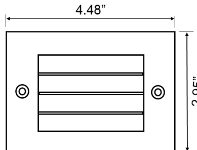
Grilled Cover with Frosted Lens
